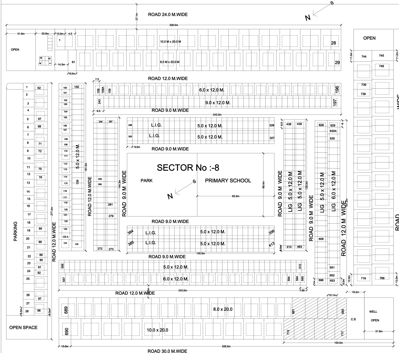
REVISED LAY OUT PLAN OF SECTOR No :-8 AT BHIWADI SCHEME(ALWAR)
