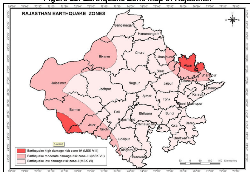
Figure 23: Earthquake Zone Map of Rajasthan
