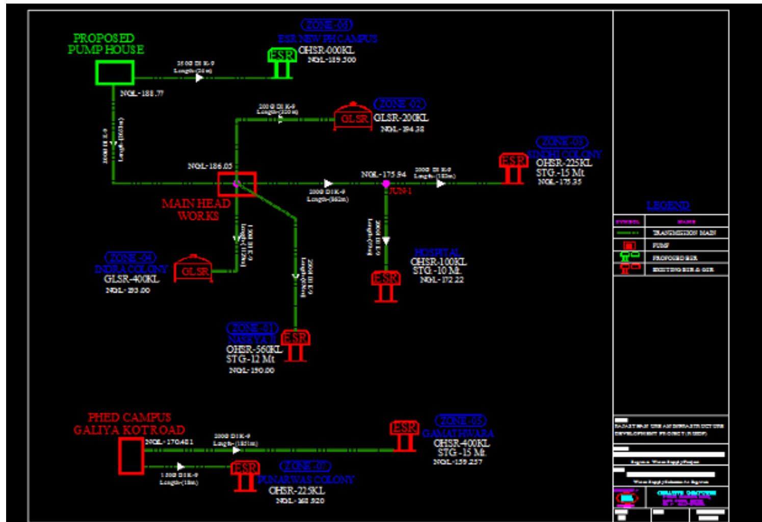
Figure 1: Flow diagram of proposed water supply works
