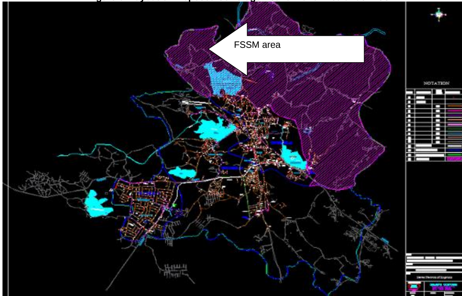
Figure 6: Layout of Proposed Sewerage Network and Area under FSSM
