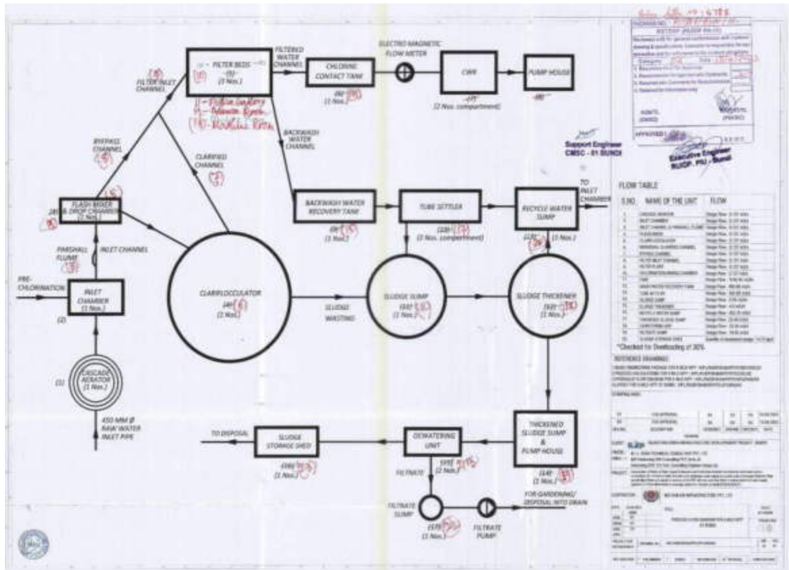
Figure 14: Approved Process Flow Diagram of 8 MLD WTP Plant in Bundi
