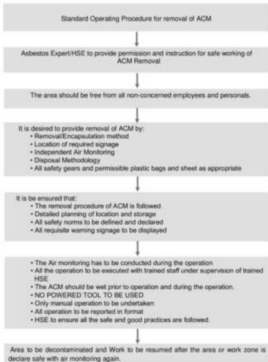
Figure 6-Standard Operating Procedure Flow Sheet
