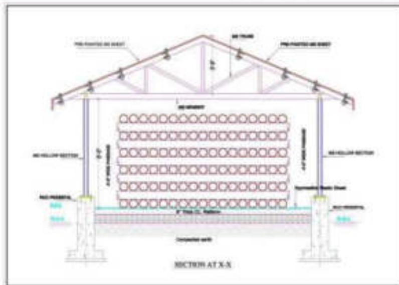
Figure 2: Schematic diagram showing ACM Pipes stacking
