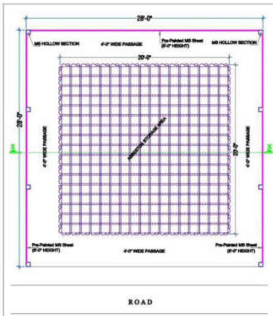
Figure 3: Schematic diagram showing ACM Pipes storage area
