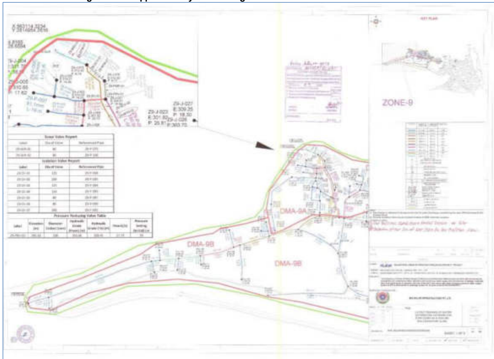
Figure 18 A: Approved Layout Drawing of Water Distribution Network for Zone-9
