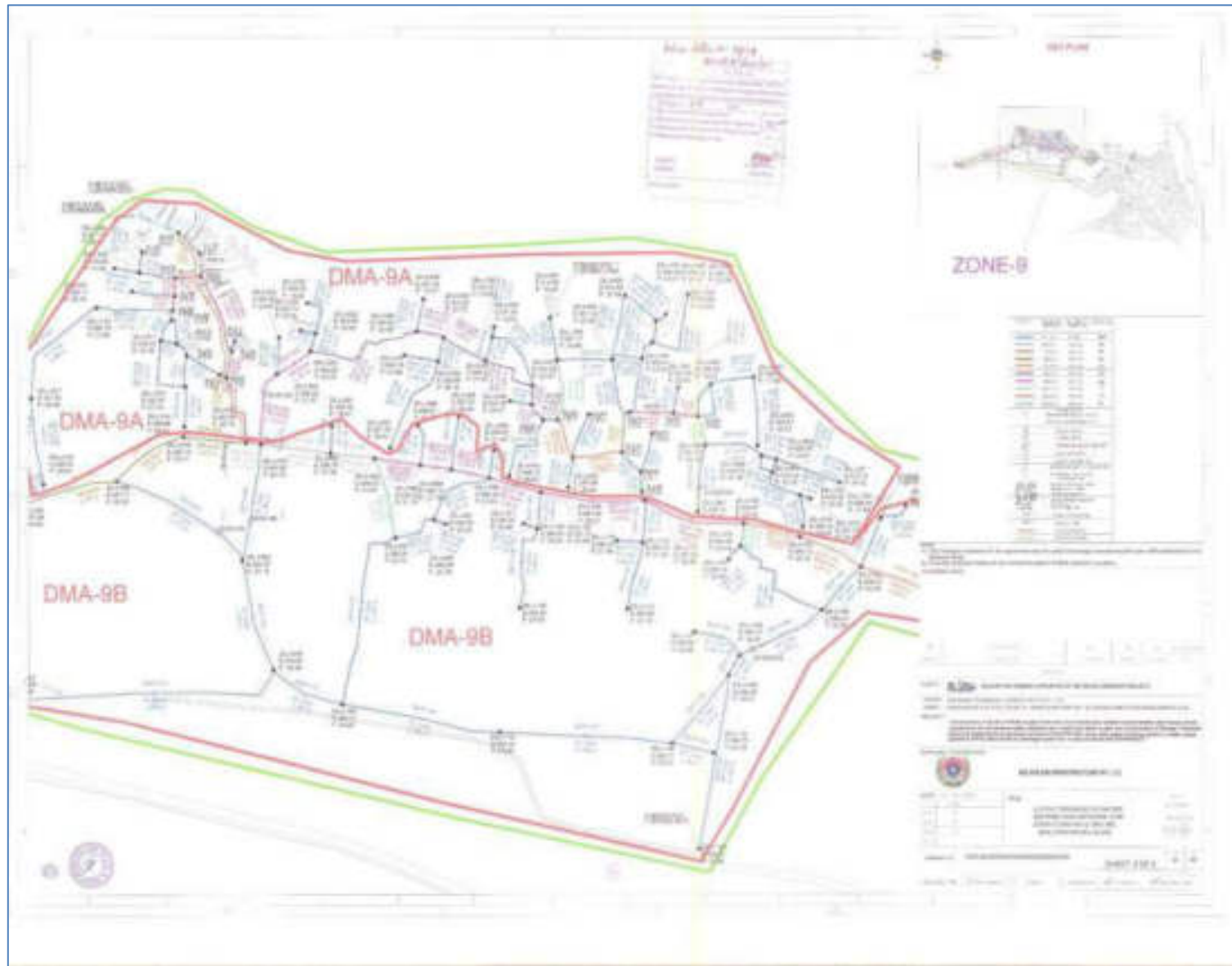
Figure 18B: Approved Layout Drawing of Water Distribution Network for Zone-9
