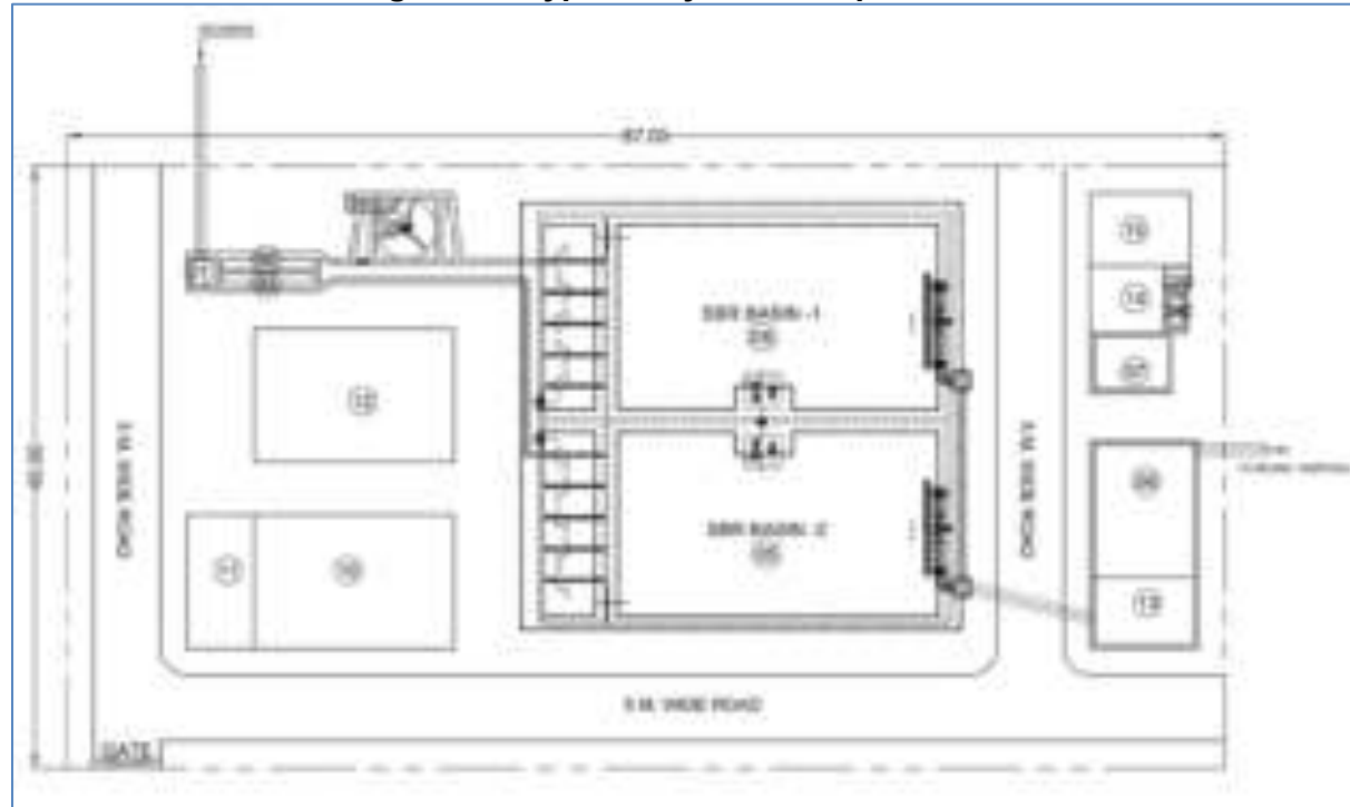
Figure 13: Typical Layout of Proposed STP
