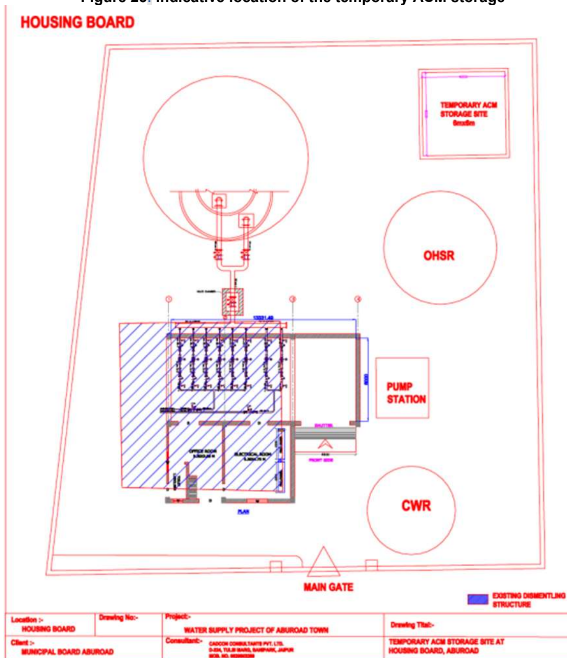
Figure 23: Indicative location of the temporary ACM storage
