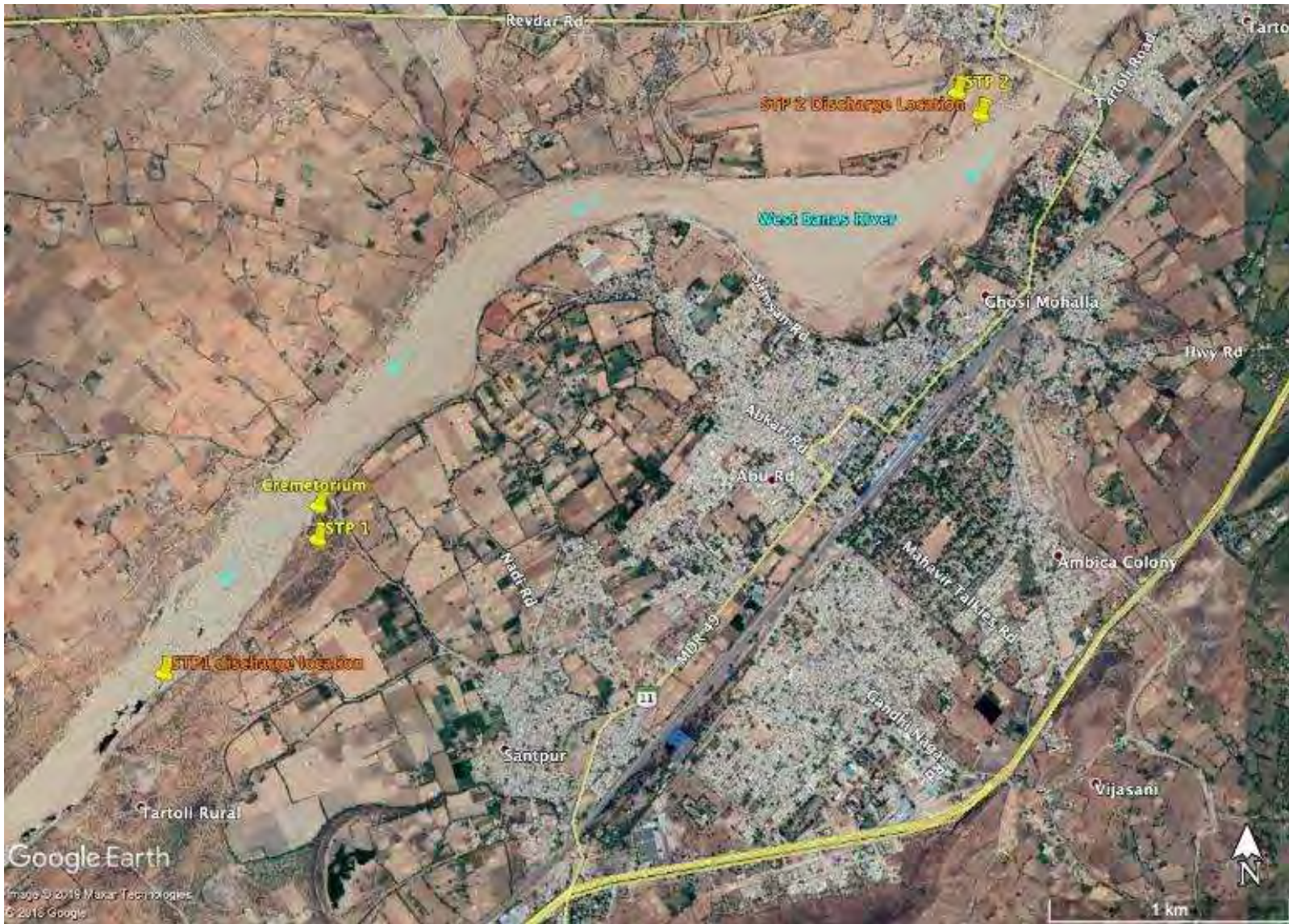
Figure 5: Location of Proposed Sewerage Components
