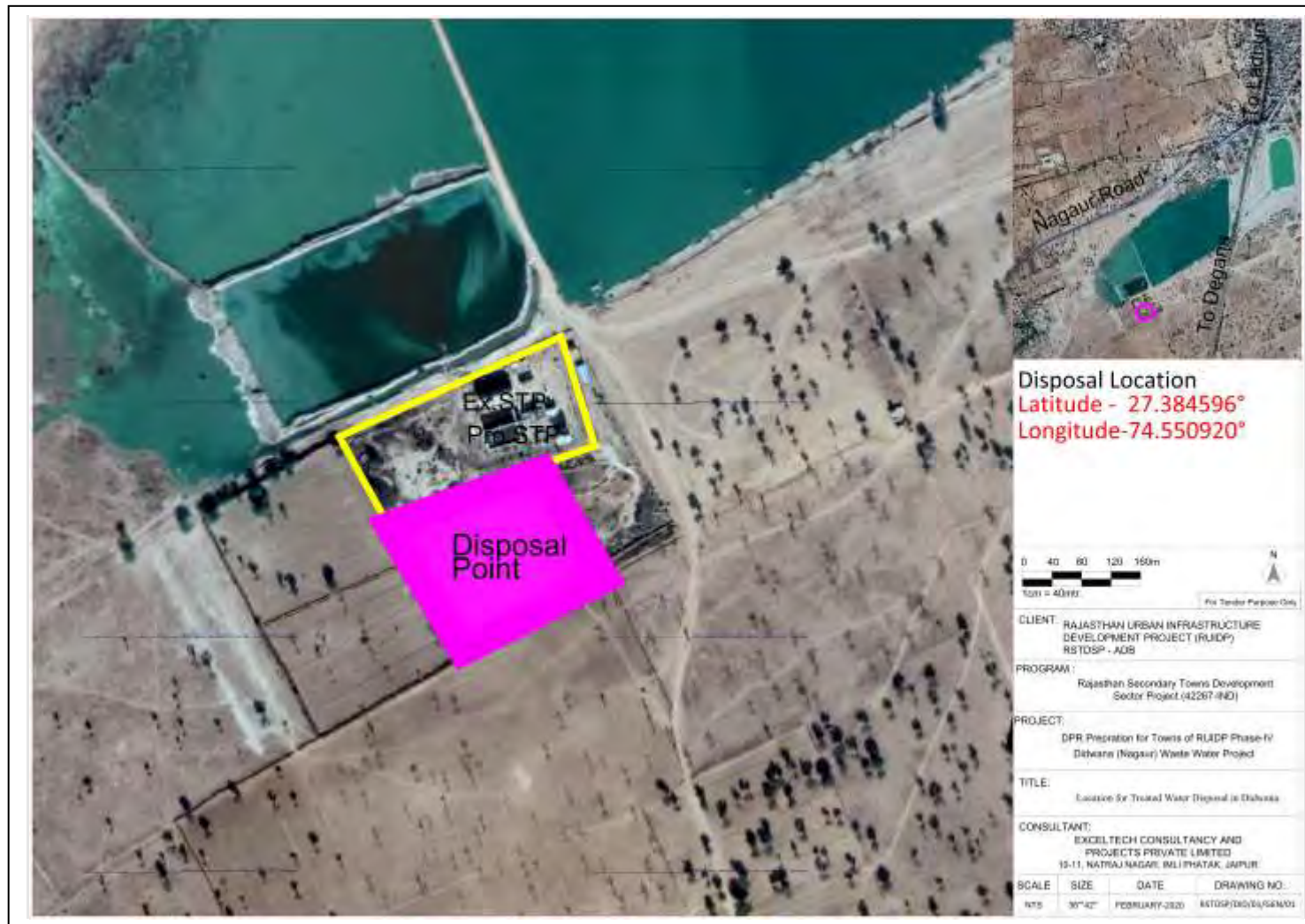
Figure 14: STP disposal map of Didwana, Rajasthan
