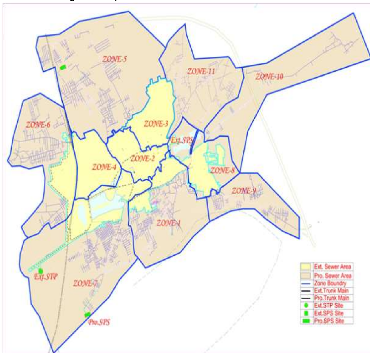
Figure 6: Proposed Sewer Networks and Zones in Didwana
