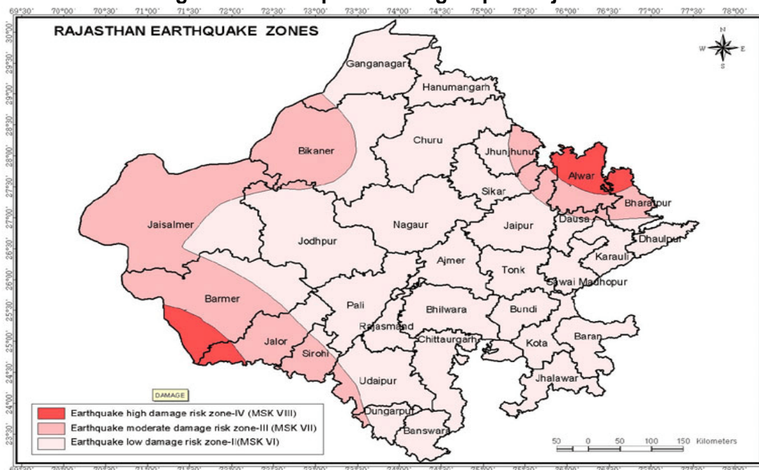
Figure 23: Earthquake Zoning Map of Rajasthan
