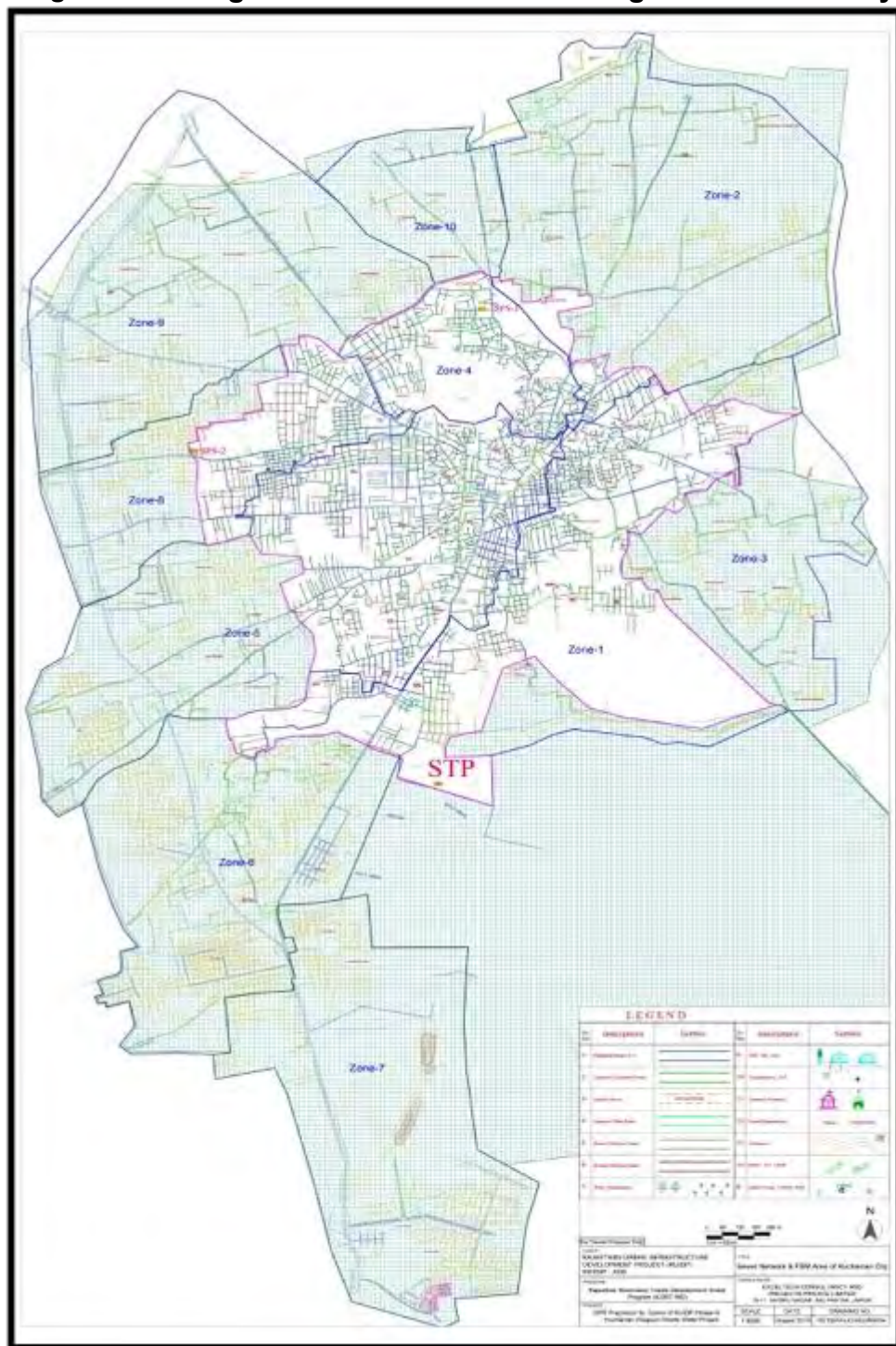
Figure 16: Designed Sewer Network Coverage–Kuchaman City
