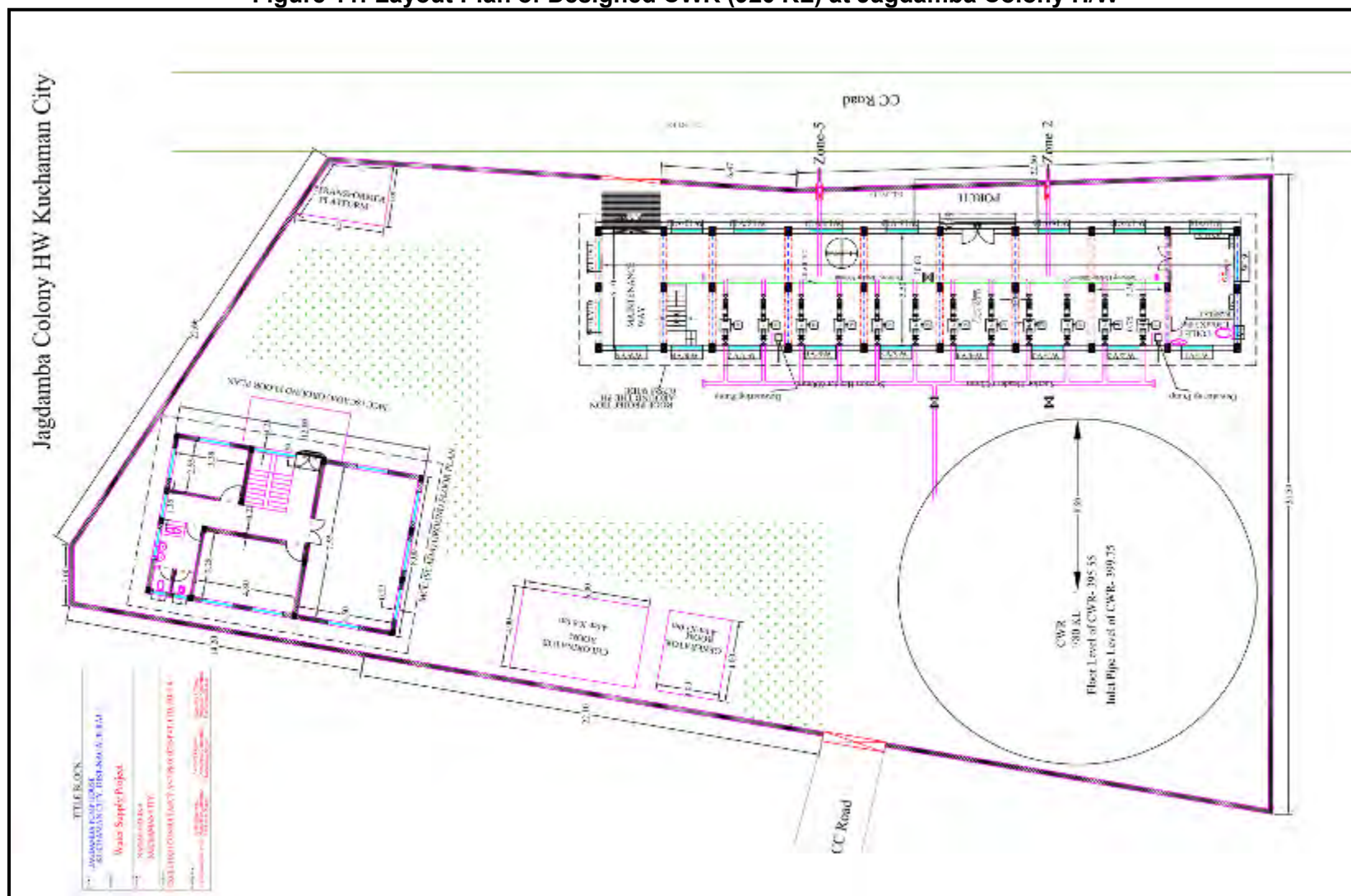
Figure 11: Layout Plan of Designed CWR (920 KL) at Jagdamba Colony H/W
