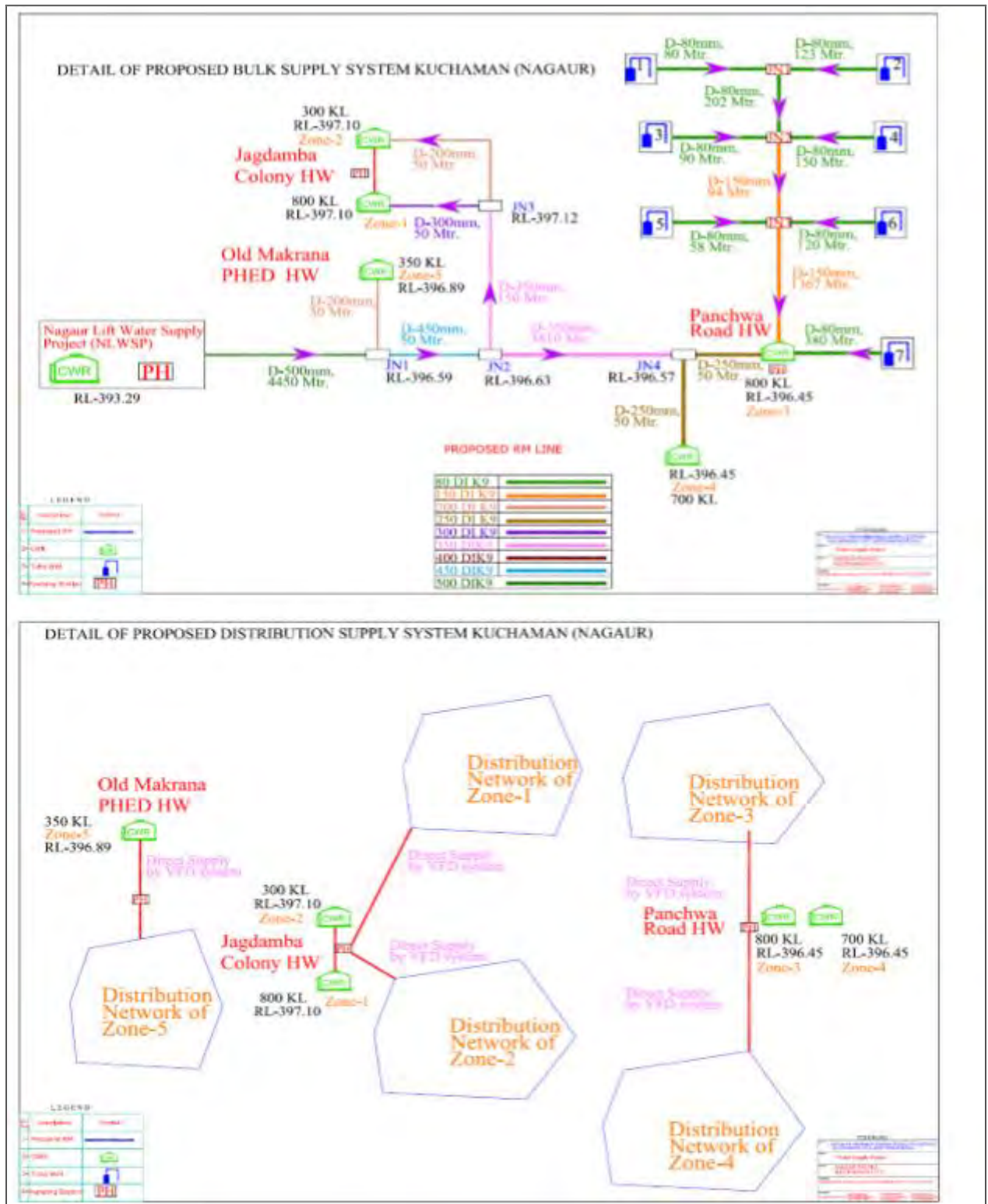
Figure 10: Designed Water Supply Distribution Network Improvement
