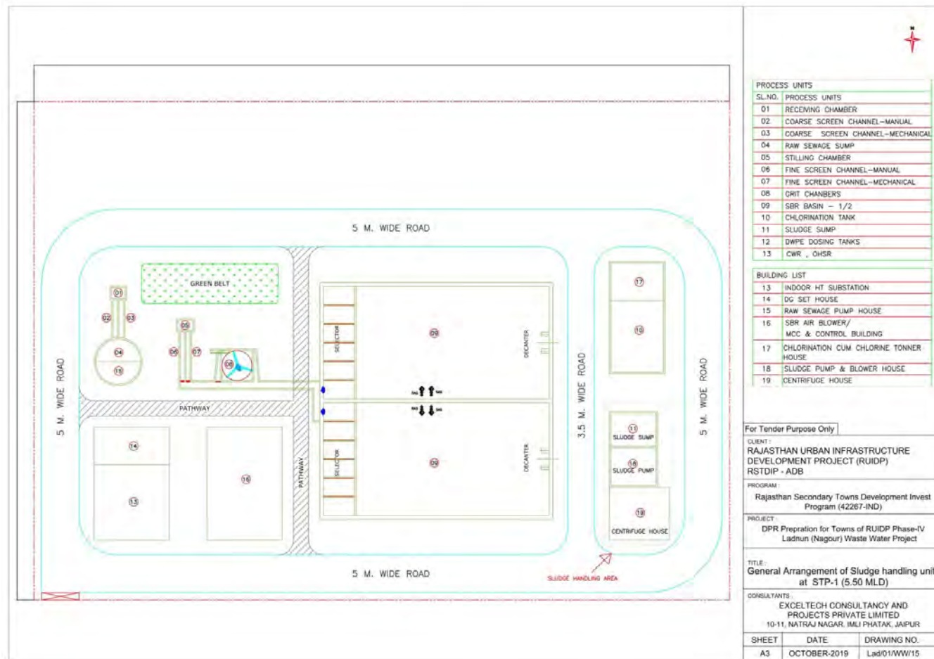
Figure 7: Layout of STP 5.5 MLD near Sri Madhav B.Ed College showing Sludge Handling Area
