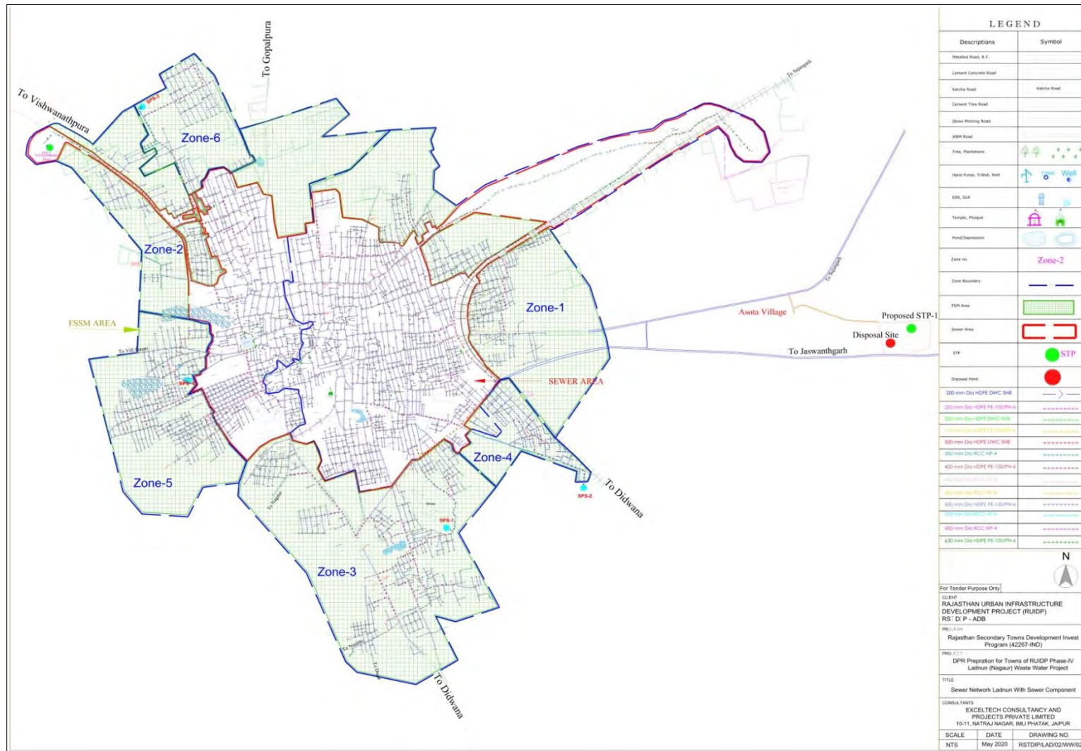
Figure 5: Layout showing of Proposed Sewerage components and FSSM Area in Ladnu
