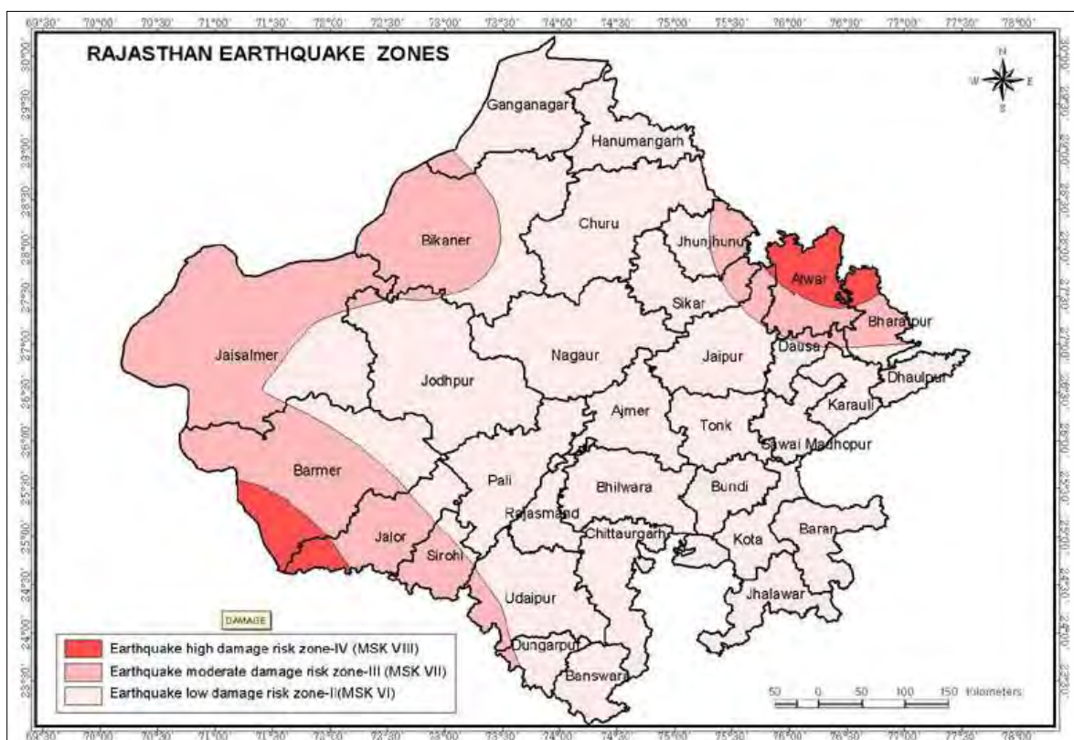
Figure 18: Earthquake Zoning Map of Rajasthan Showing Project Area
