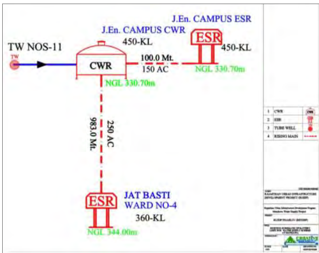
Figure 1: Flow Diagram of Existing Water Supply System in Mandawa
