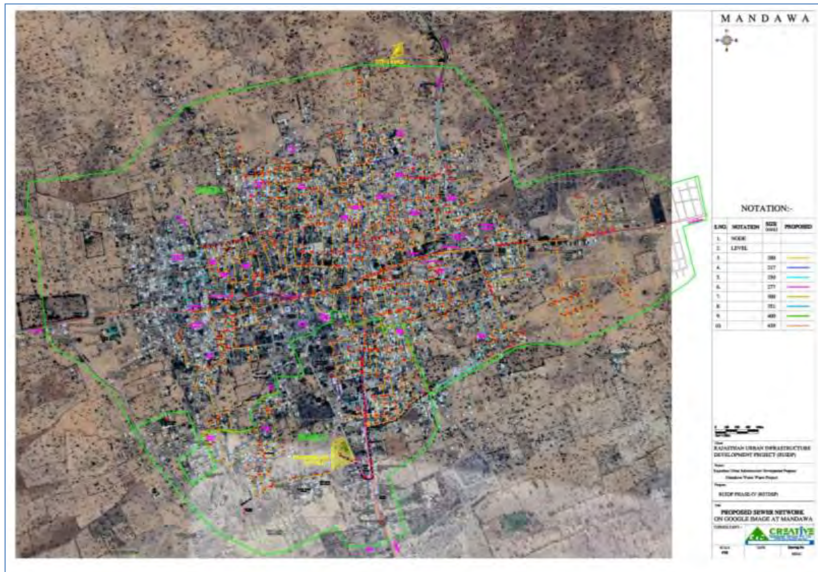
Figure 12: Proposed Sewerage Component on Google – Mandawa town
