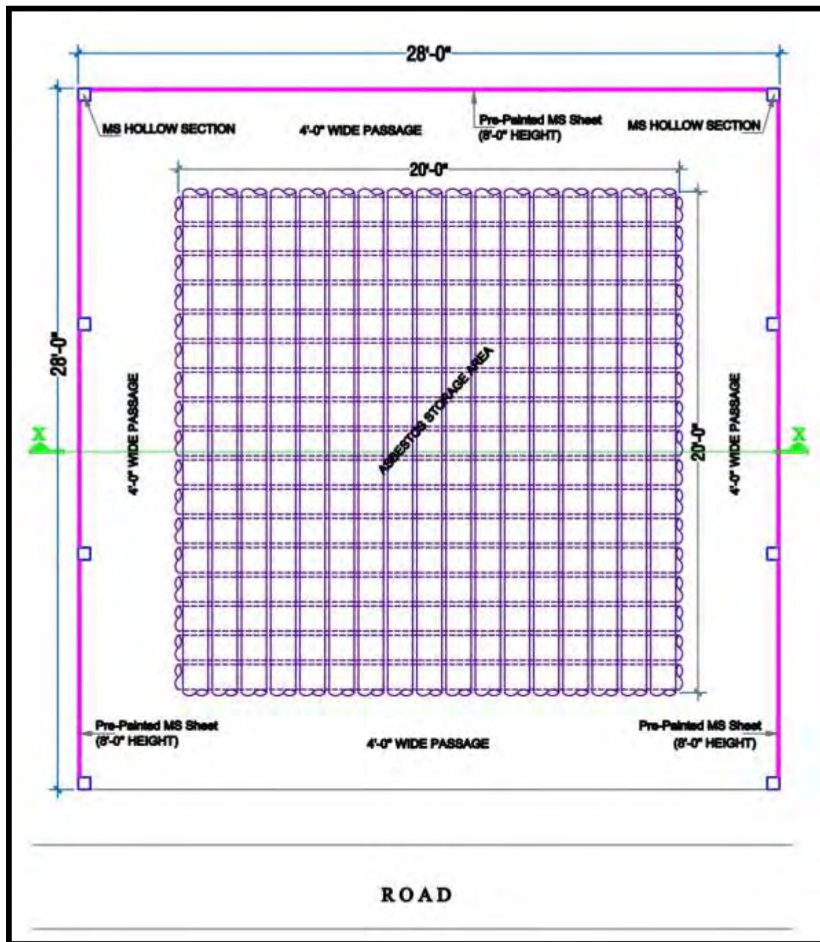
Figure 3: Schematic diagram showing ACM Pipes storage area
