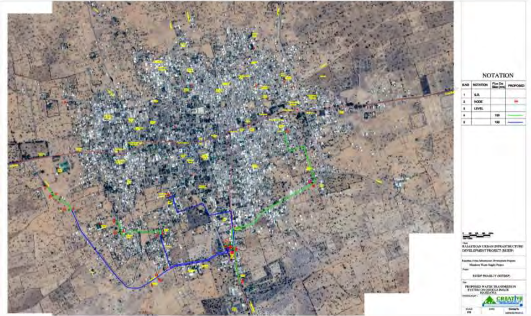
Figure 9: Layout of Proposed Water Transmission System on Google – Mandawa town
