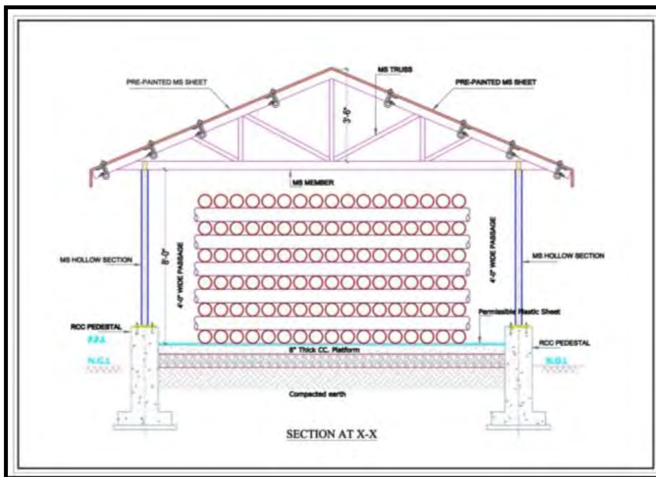
Figure 2: Schematic Diagram Showing ACM Pipe Stacking
