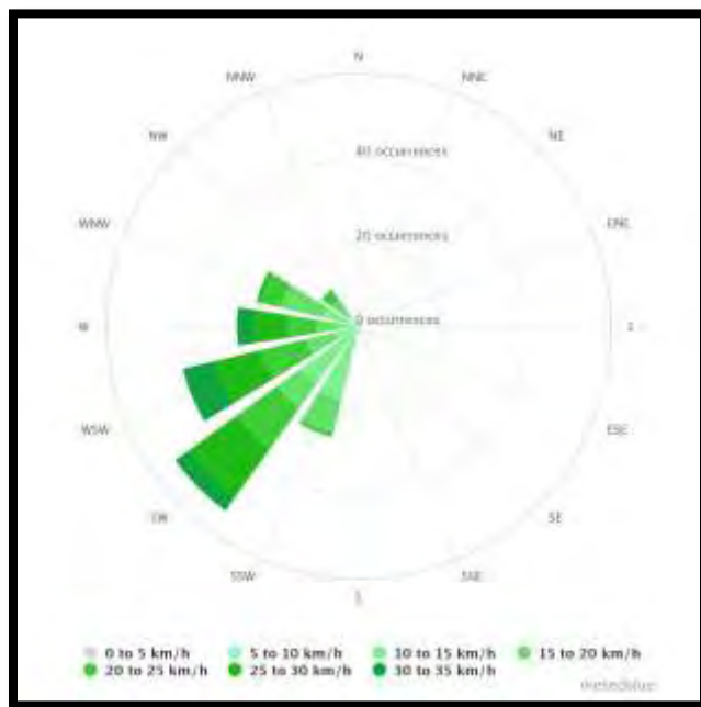
Figure 7: Predominant Wind Direction in Mandawa, District-Jhunjhunu, Rajasthan
