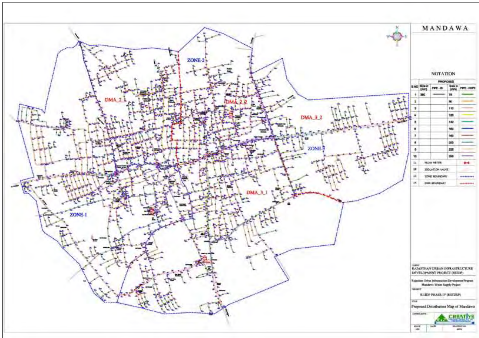
Figure 7: Proposed Water Supply Distribution Network Improvement
