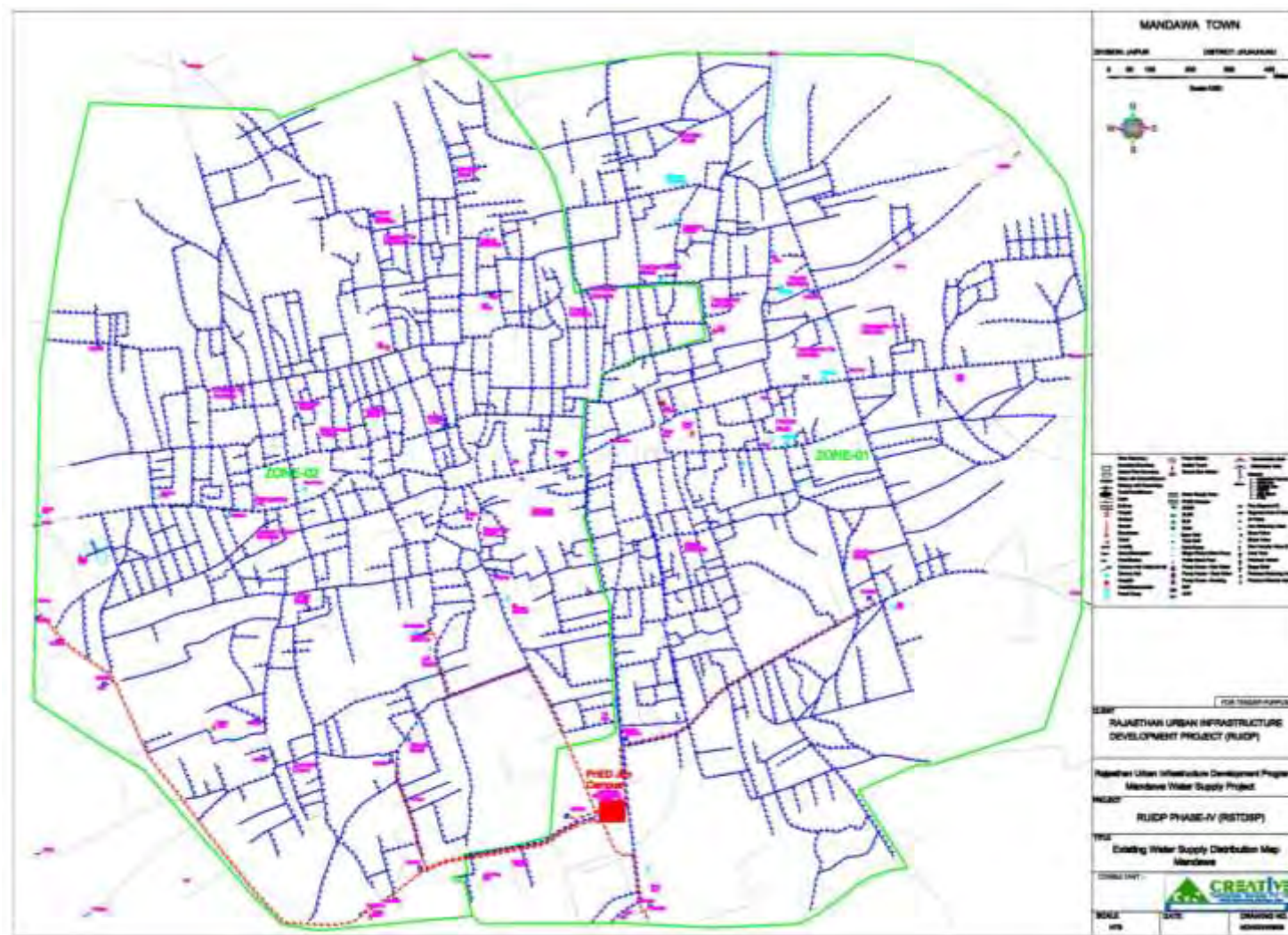
Figure 2: Existing Water Supply distribution and component Map (Composite Map) of Mandawa
