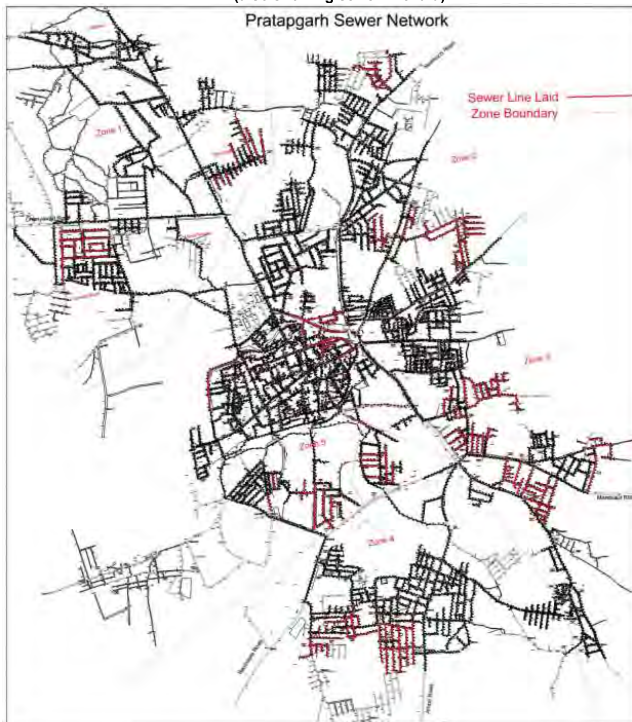
Figure 5: Approved Layout of Sewerage Networks in Pratapgarh (also showing sewer line laid)
