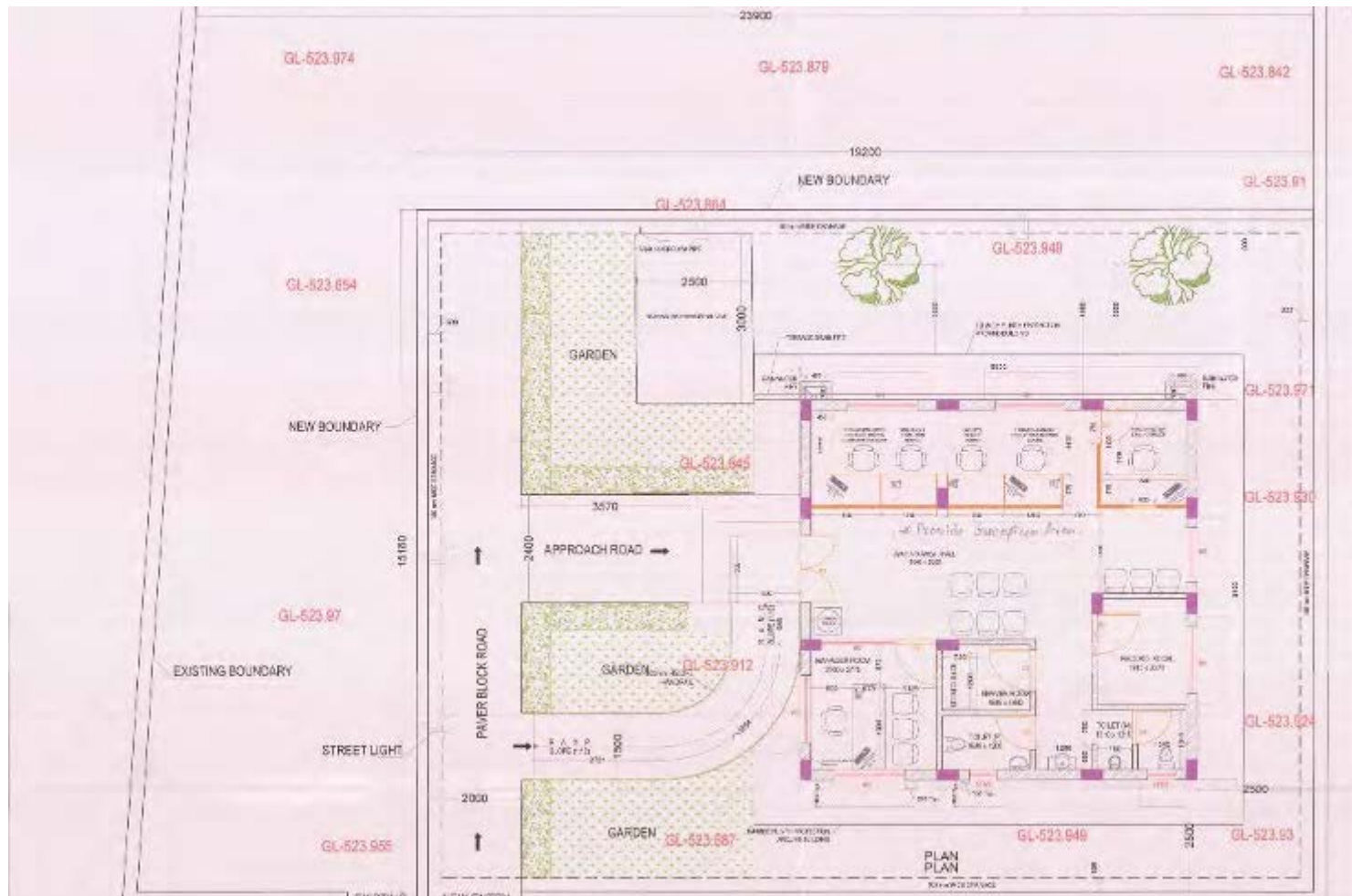
Figure 4: Layout of Proposed CRMC
