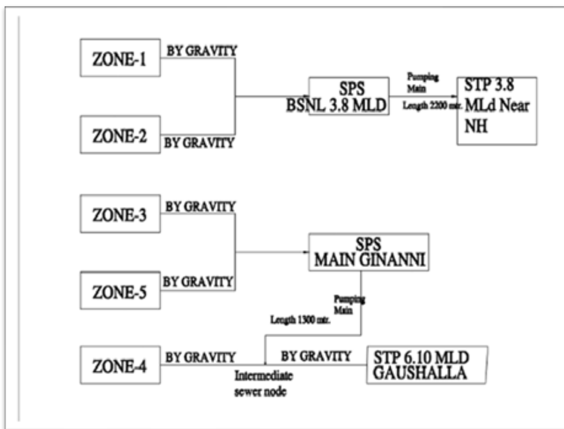
Figure 1: Schematic Diagram of Proposed Works
