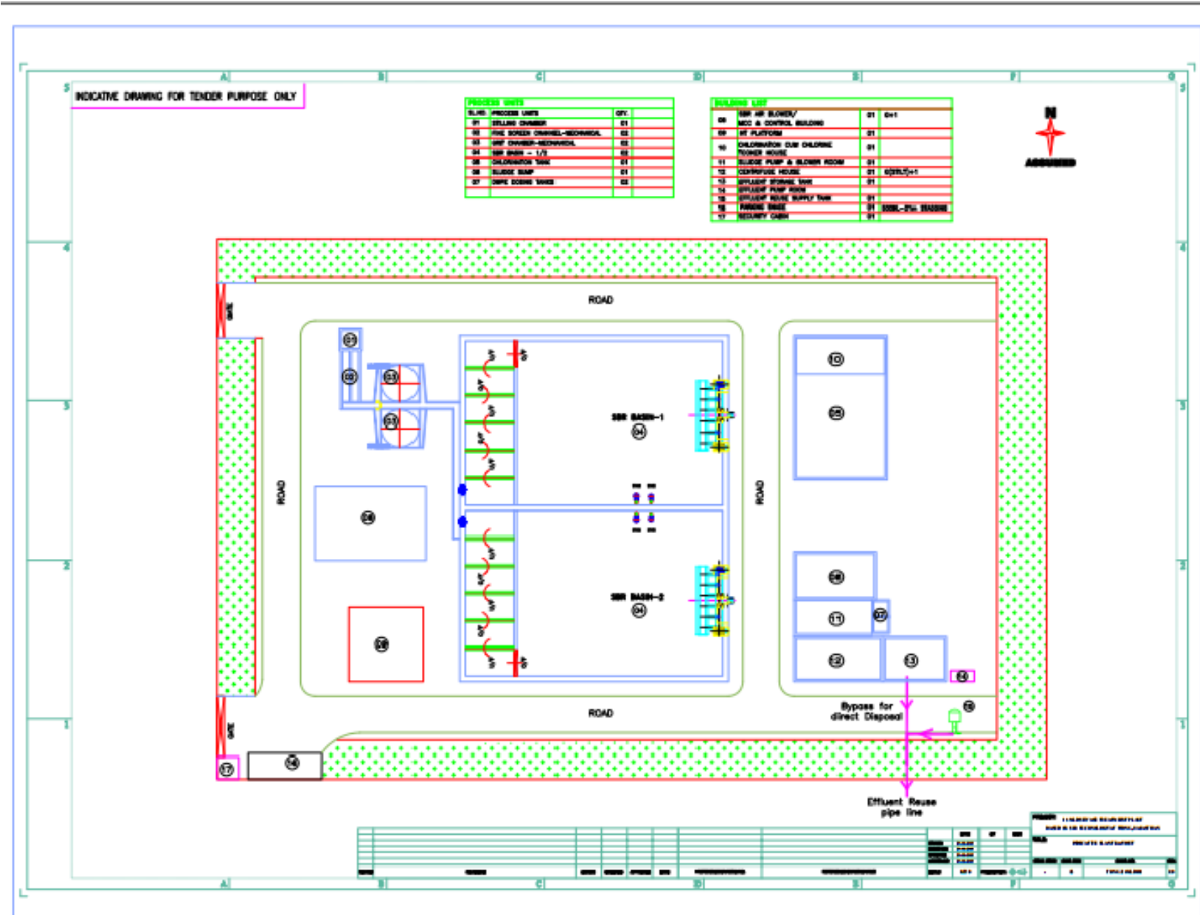
Figure 6B: Layout Map of Proposed STP 16 MLD
