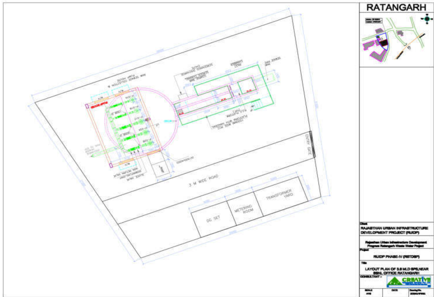
Figure 14: Layout Plan for Proposed SPS 1 near BSNL Office
