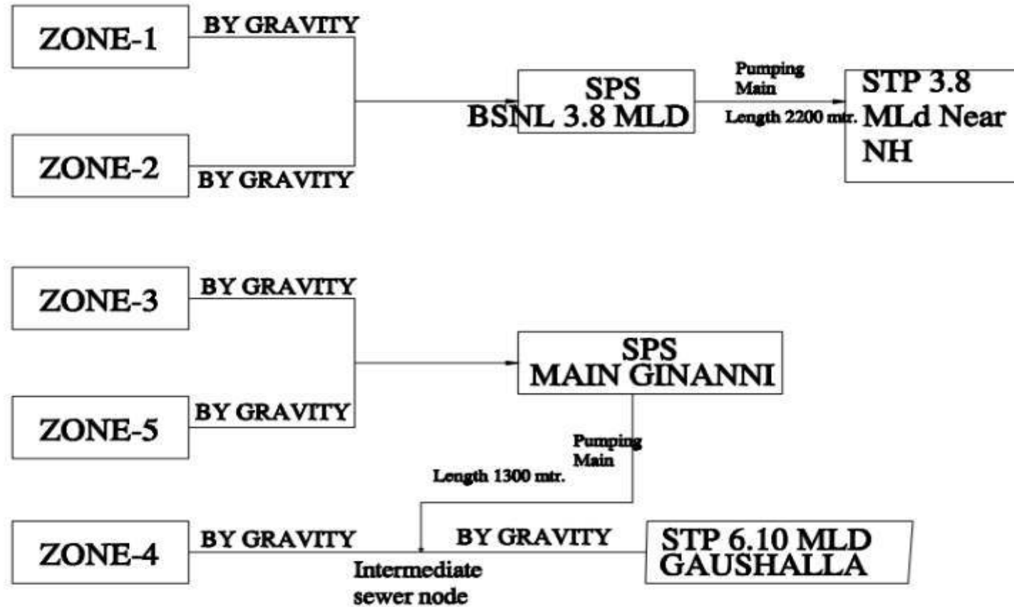
Figure 1: Schematic Diagram of Proposed Works
