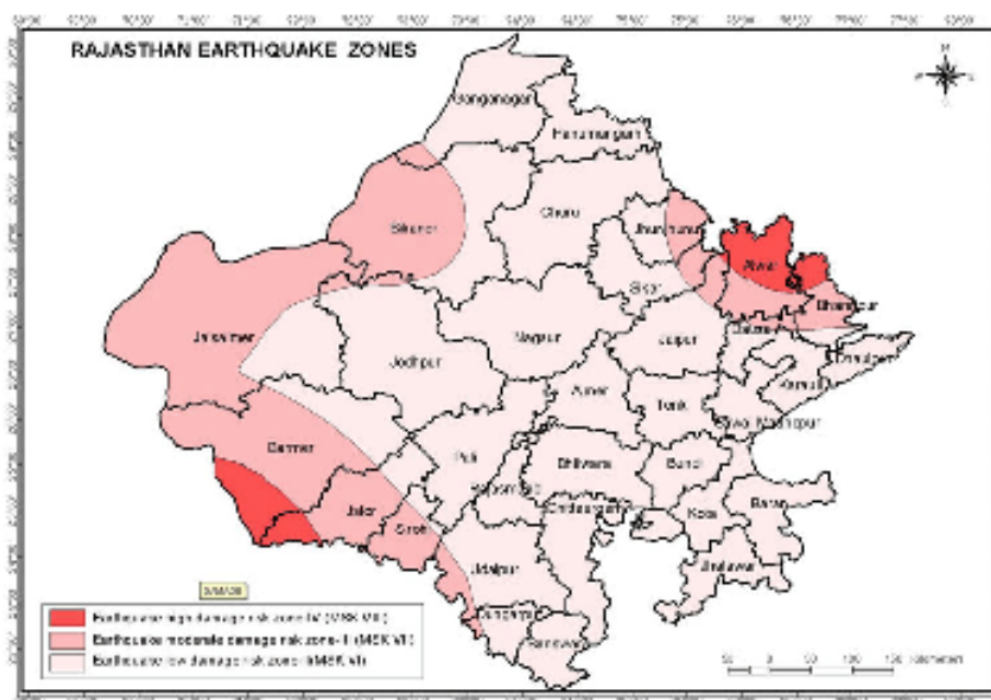
Figure 11: Earthquake Zoning Map of Rajasthan Showing Project Area
