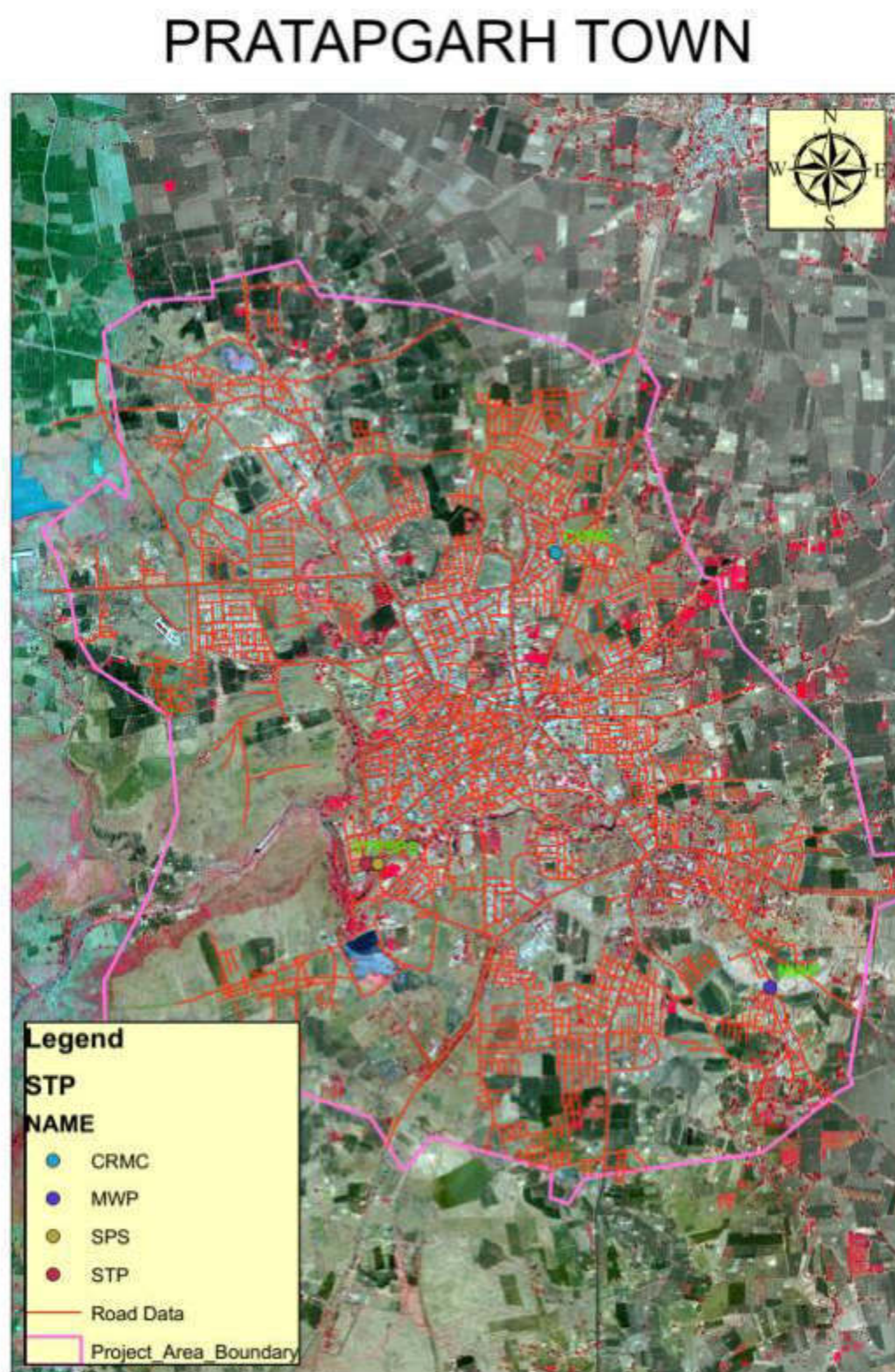
Figure 4A: Location of Proposed STP, SPS, MWP and CRMC in Pratapgah town
