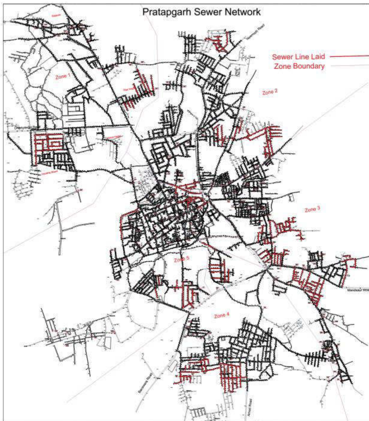
Figure 5: Approved Layout of Sewerage Networks in Pratapgarh
