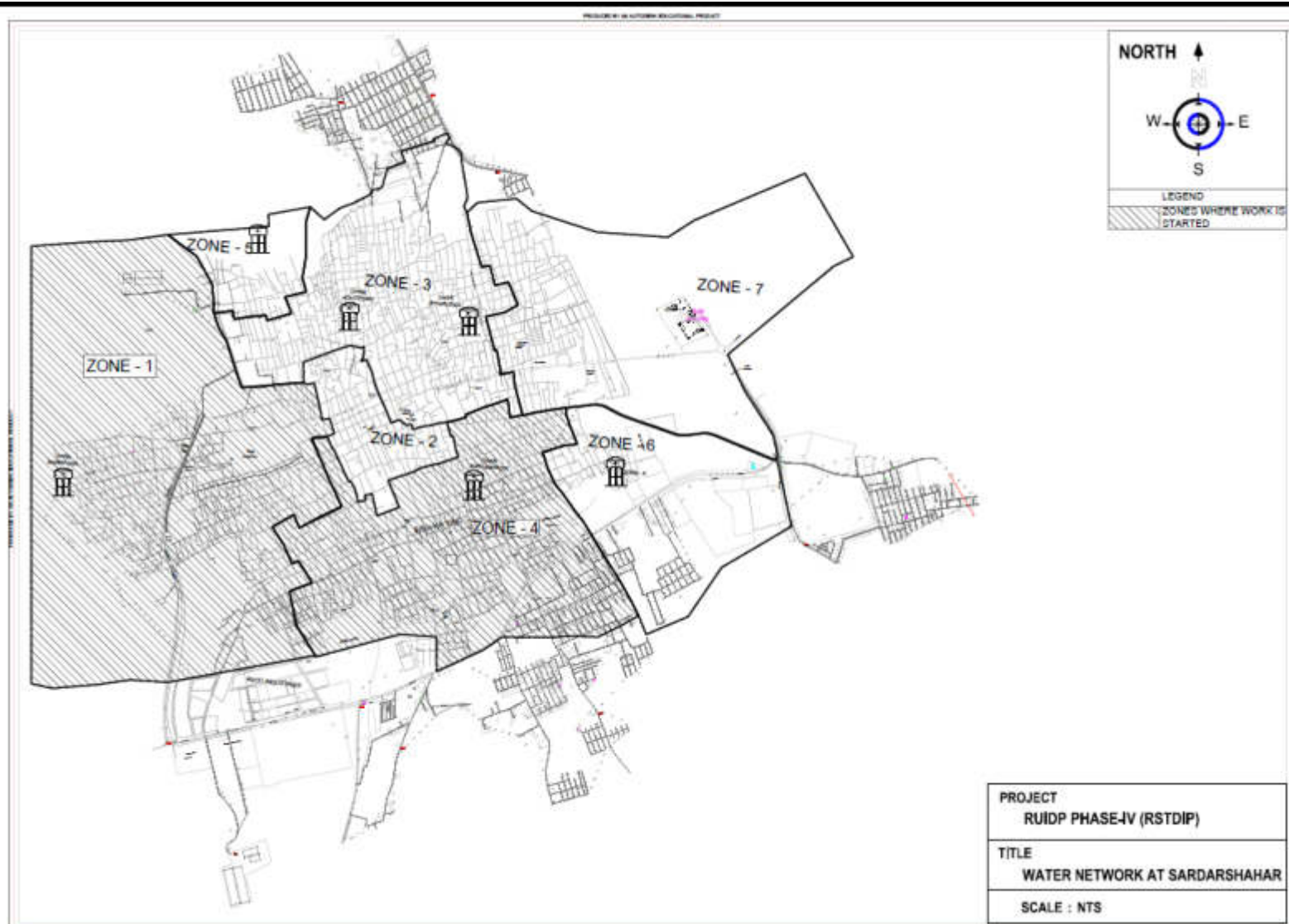
Water Supply Network Map showing approved Zones 1 and 4
