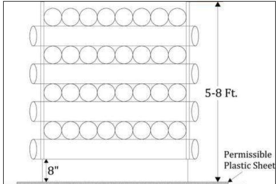
Fig.No.5: Schematic diagram showing ACM Pipes stacking
