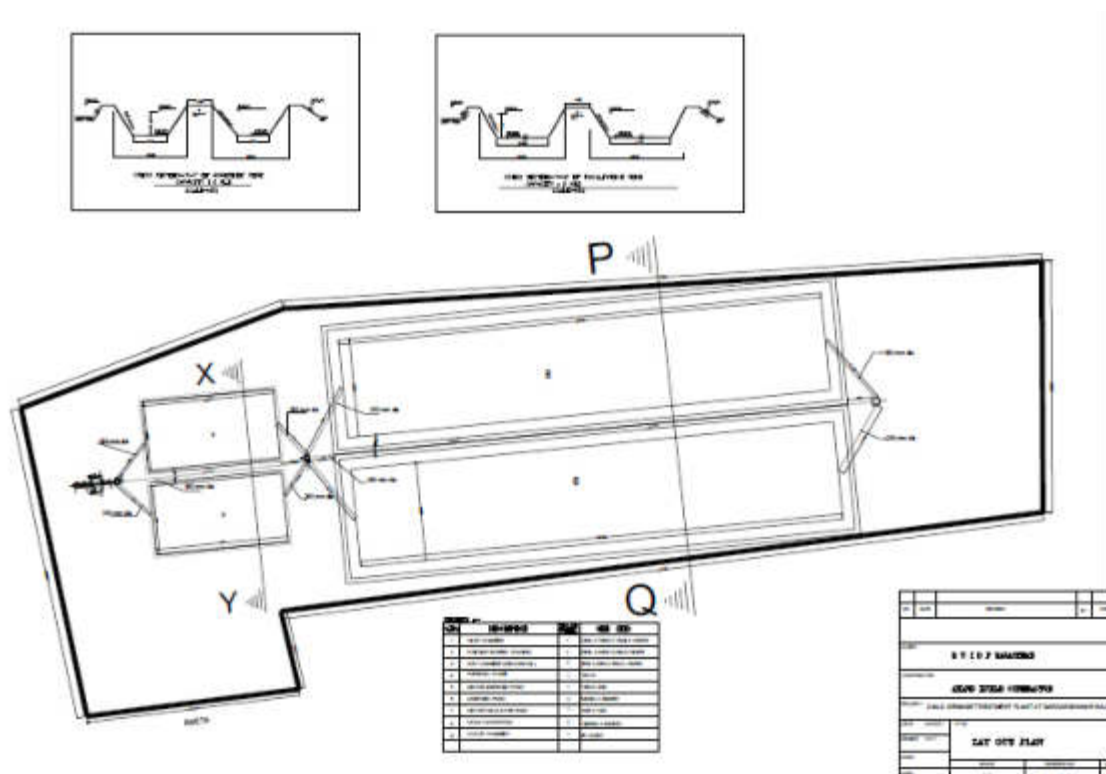
Layout of 05 MLD STP (Existing) – South
