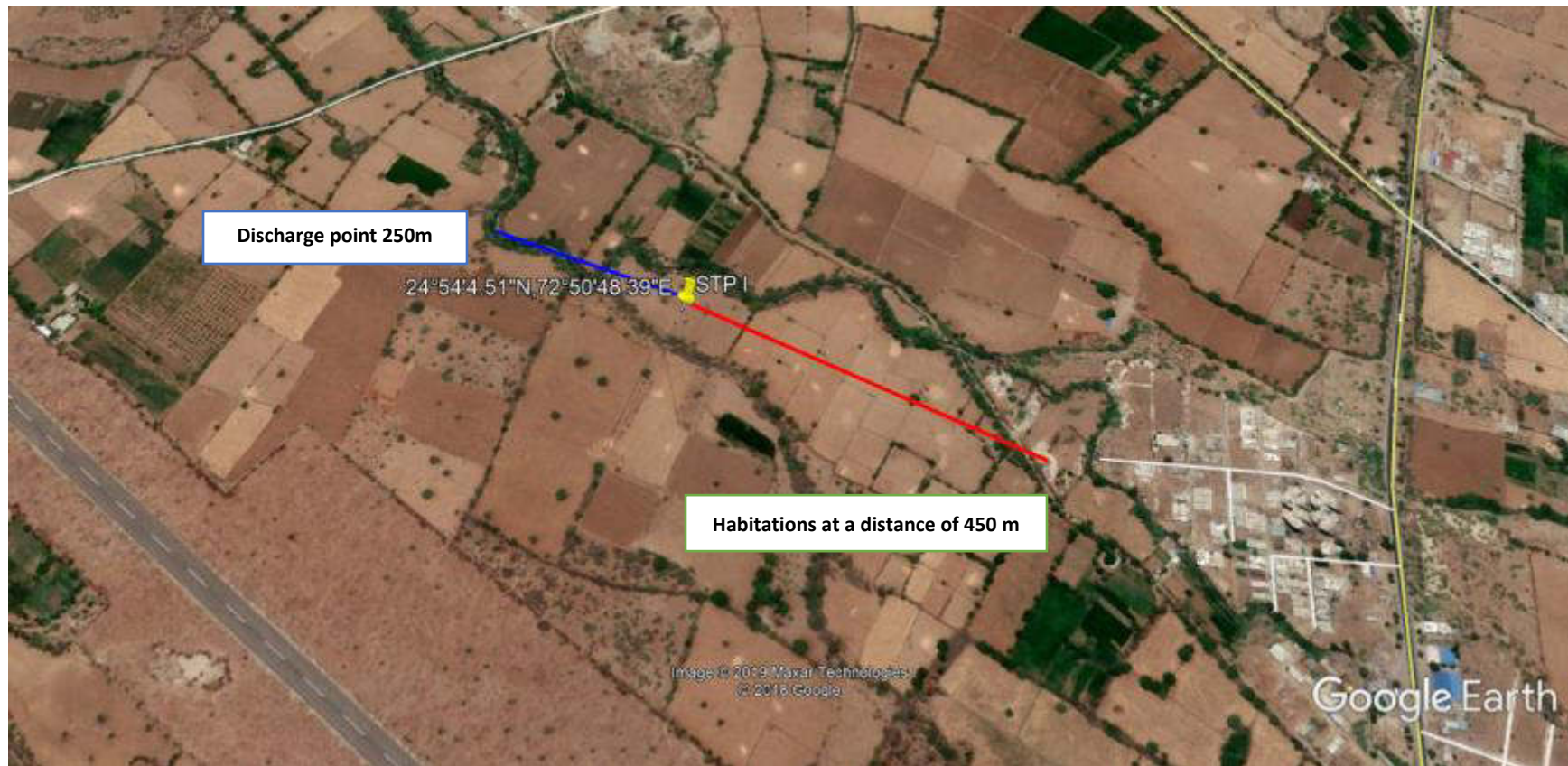
Figure 18: Location of STP Site 1 and Discharge Pont
