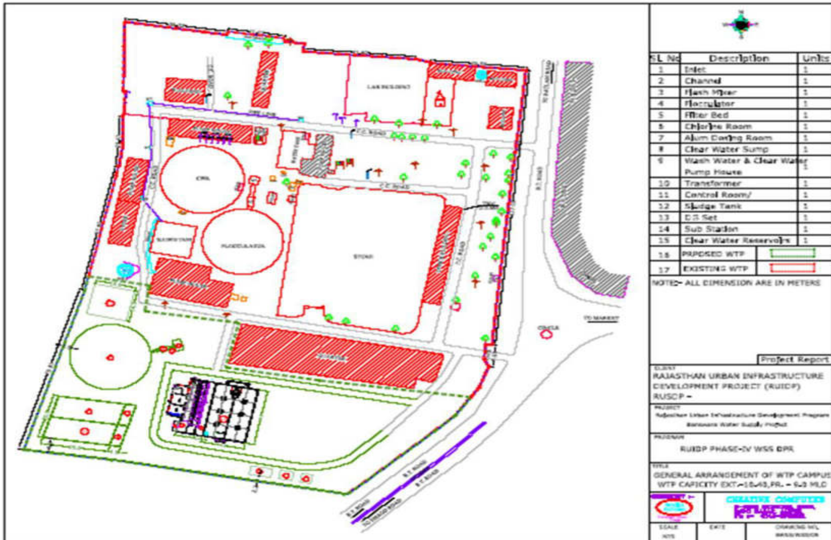
Figure 4: Conceptual Layout Plan of Proposed WTP
