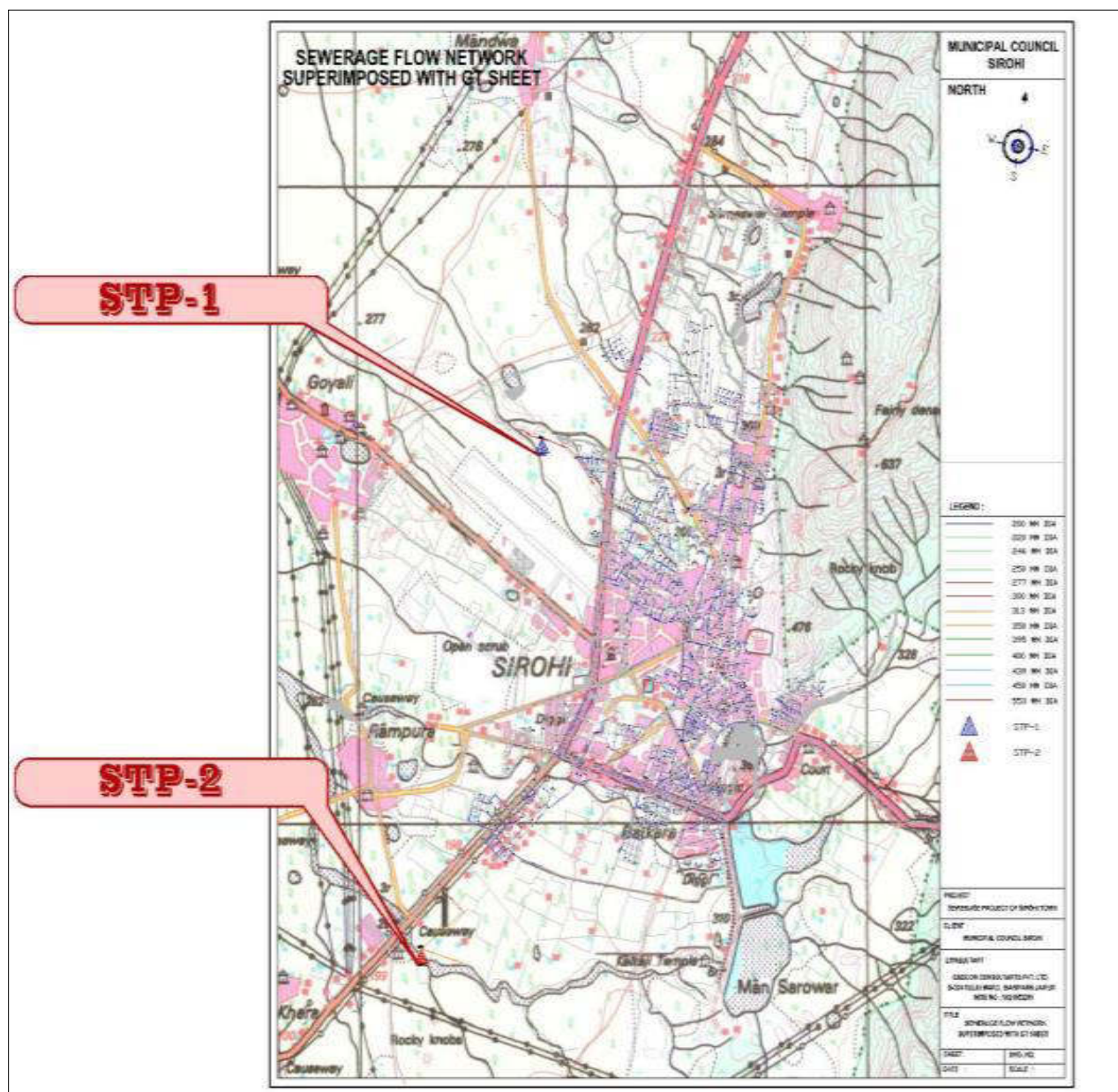
Figure 8: Proposed Sewer Network Coverage on SOI Toposheet
