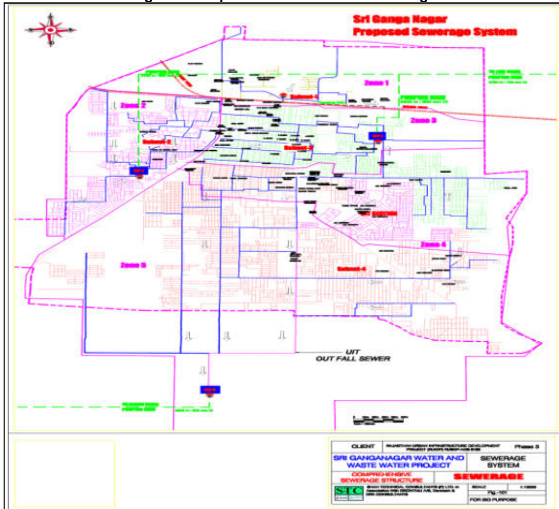
Figure 2: Proposed Sewer Network Coverage
